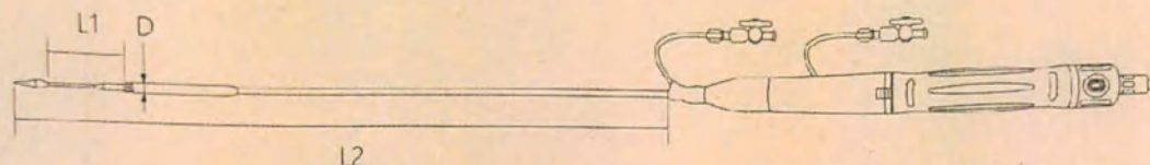
Transcatheter Aortic Valve Replacement Retrieable Delivery System
