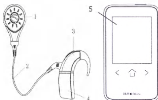
1 Transmission Coil; 2 Transmitting wire; 3 Signal processing unit; 4 BTE rechargeable battery compartment; 5 Remote control
