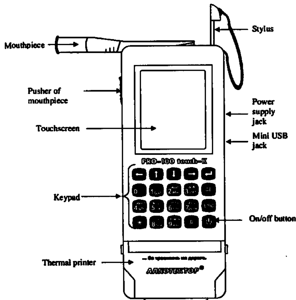
Figure 1 – Analyzer appearance
