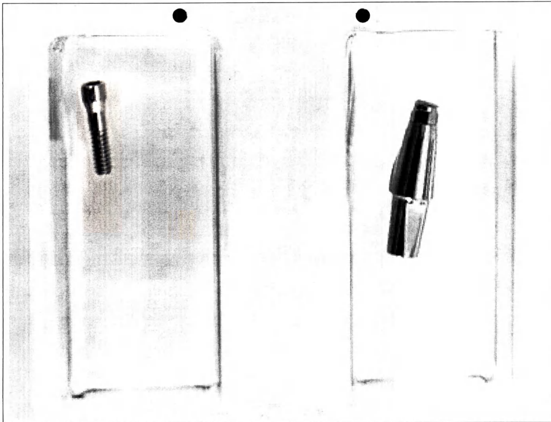
Абатмент Implantswiss Bone Level Mini Couple Abutment, Dimensions: Diameter - 3.7 mm, Gingival Height - 4.0 mm NON STERILE (артикул S-BMCA3740)
