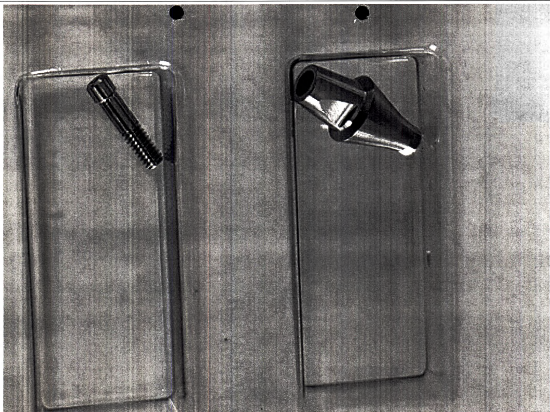
Абатмент Implantswiss Bone Level Couple Abutment, Dimensions: Diameter - 6.5 mm, Gingival Height - 5.0 mm, Over Gingival Margin Height - 7.0 mm NON STERILE (артикул S-BCA65507)
