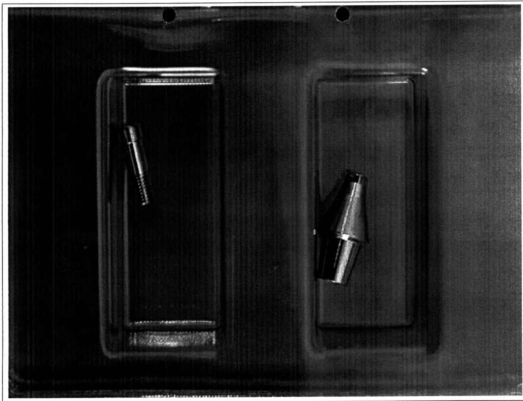
Абатмент Implantswiss Bone Level Couple Abutment, Dimensions: Diameter - 6.5 mm, Gingival Height - 5.0 mm NON STERILE (артикул S-BCA6550)
