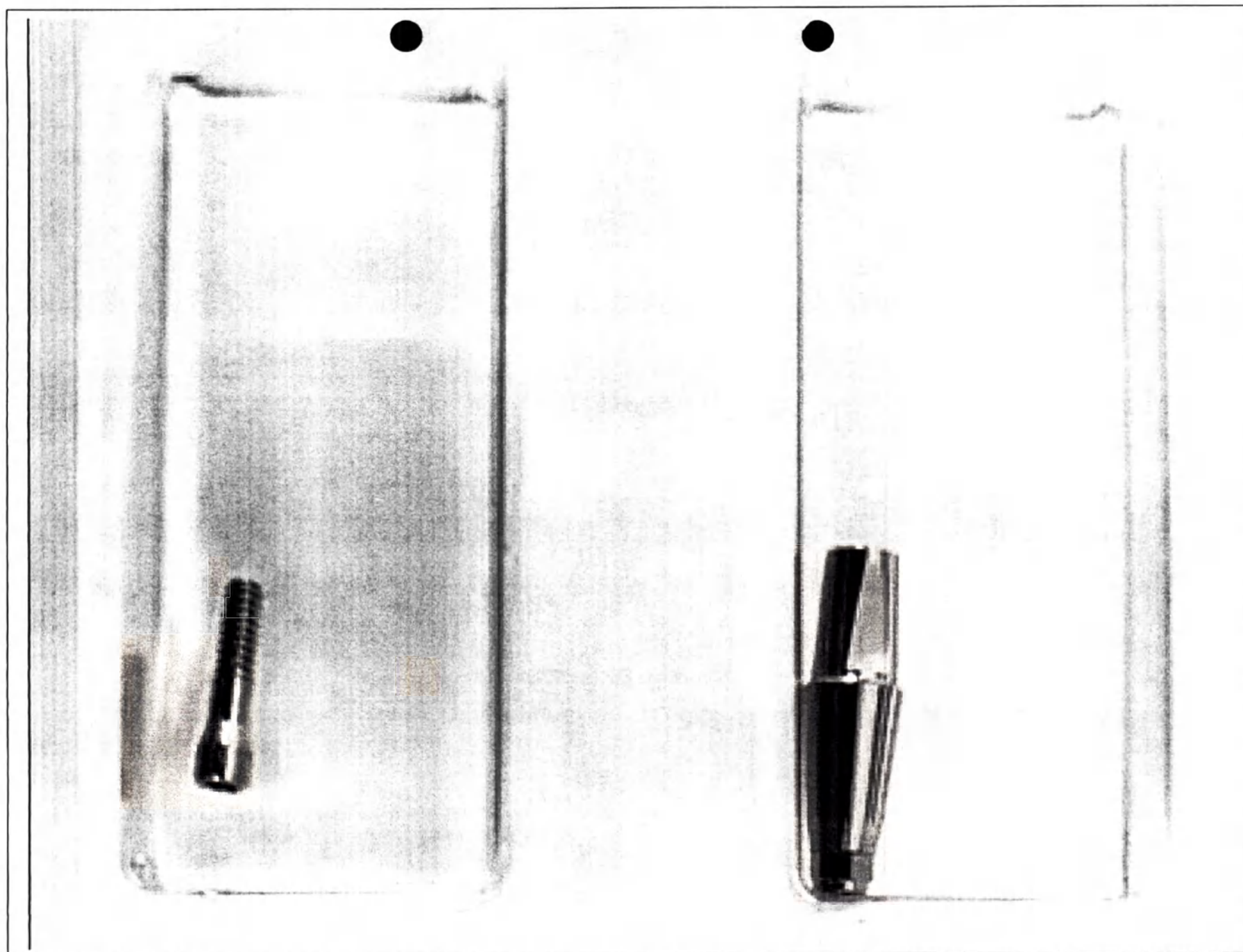
Абатмент Implantswiss Bone Level Mini Couple Abutment, Dimensions: Diameter - 3.7 mm, Gingival Height - 3.0 mm NON STERILE (артикул S-BMCA3730)
