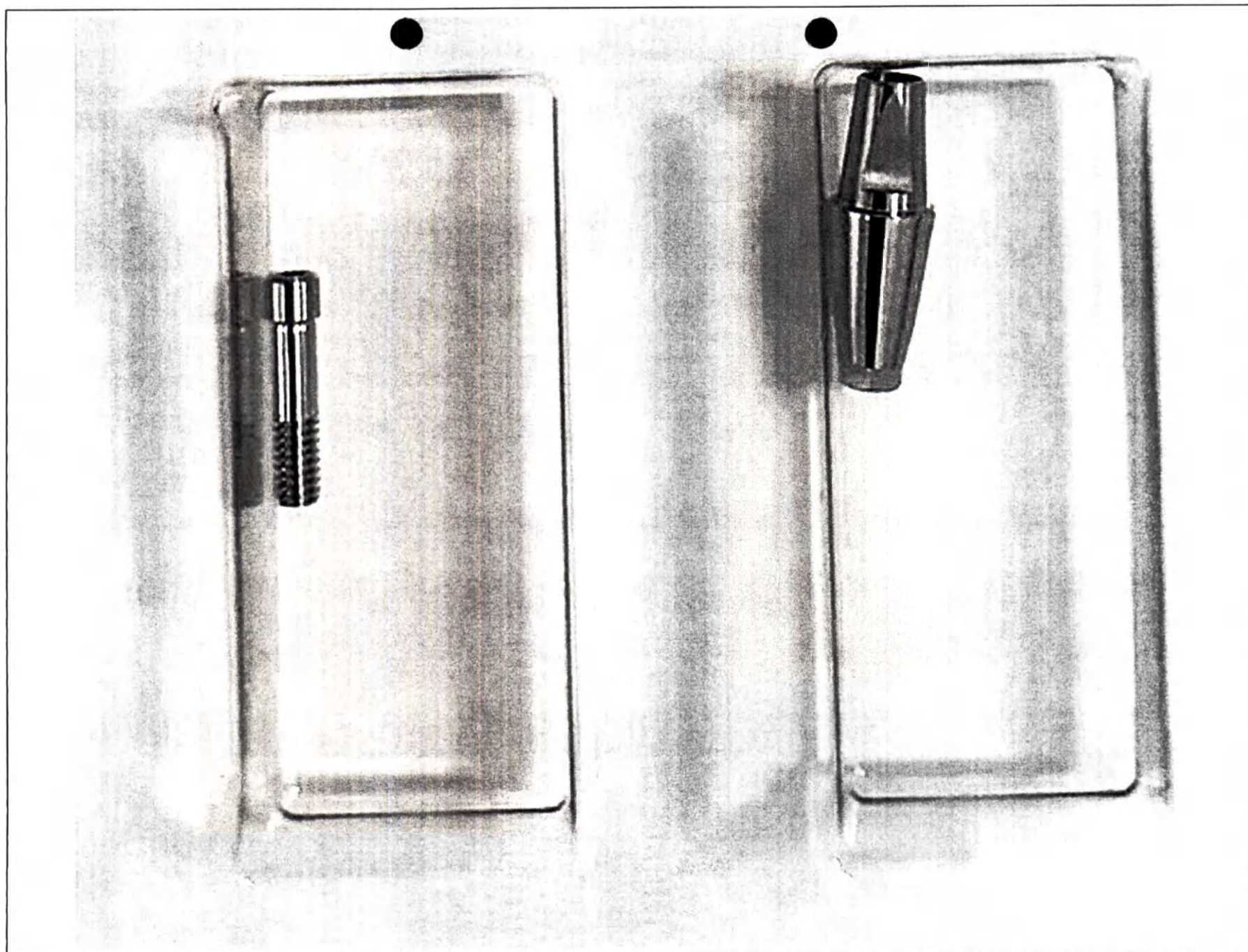
Абатмент Implantswiss Bone Level Couple Abutment, Dimensions: Diameter - 4.5 mm, Gingival Height - 2.0 mm NON STERILE (артикул S-BCA4520)
