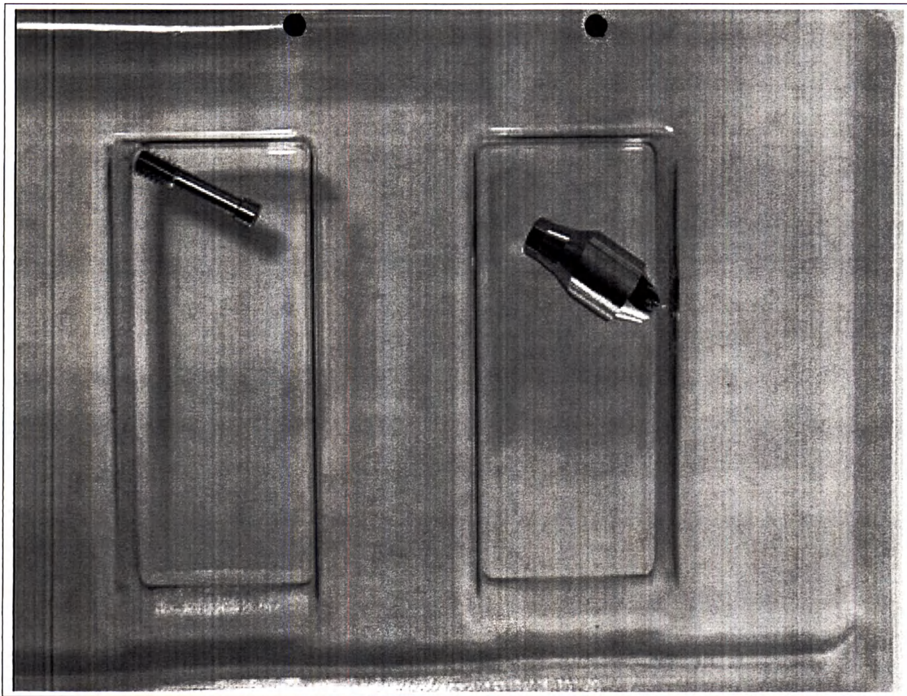
Абатмент Implantswiss Bone Level Multi Unit Abutment, Dimensions: Diameter - 4.8 mm, Angle - 17°, Gingival Height - 3.5 mm NON STERILE (артикул S-BMUA48173)
