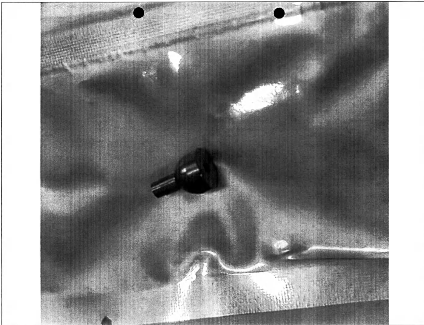
Абатмент i-system Healing Abutment, Dimensions: Diameter - 6.5 mm, Length - 6.5 mm, Well - 3.0 mm NON STERILE (артикул I-SHA6065(3))
