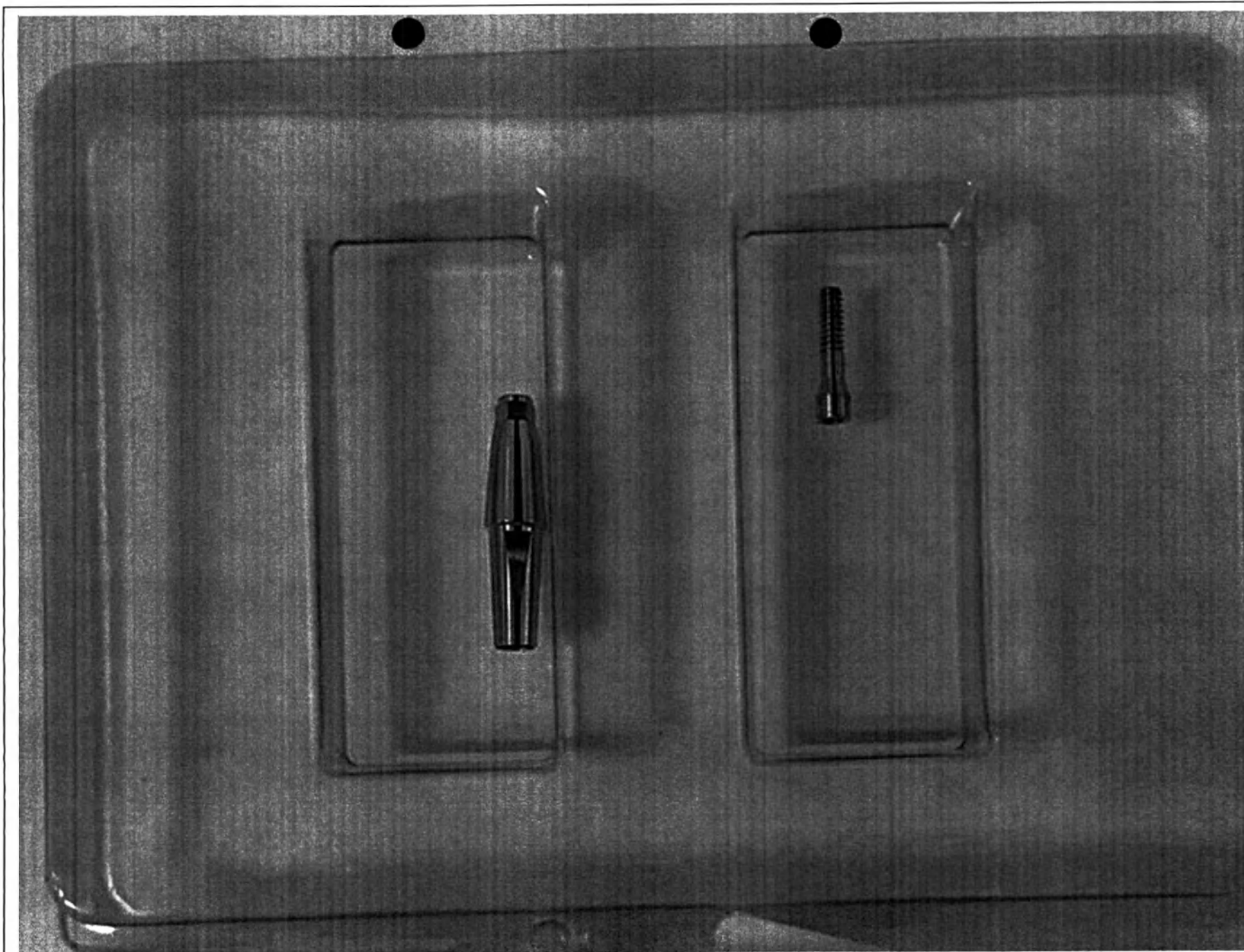
Абатмент Implantswiss Bone Level Mini Couple Abutment, Dimensions: Diameter - 3.7 mm, Gingival Height - 1.0 mm, Over Gingival Margin Height - 7.0 mm NON STERILE (артикул S-BMCA37107)
