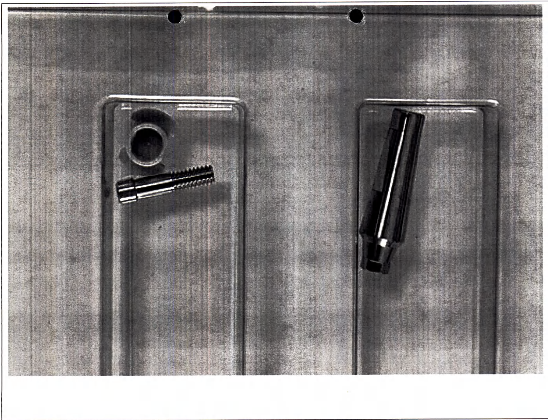
Абатмент Implantswiss Bone Level Multi Abutment, Dimensions: Diameter - 4.5 mm, Gingival Height - 1.0 mm NON STERILE (артикул S-BMA45)
