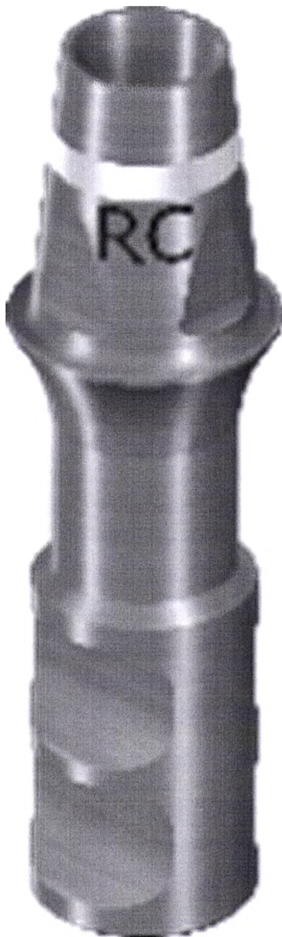
7.10. RC Implant Analog, for Cementable Abutment, D 5mm, AH 5.5mm, артикульный номер 025.4136
