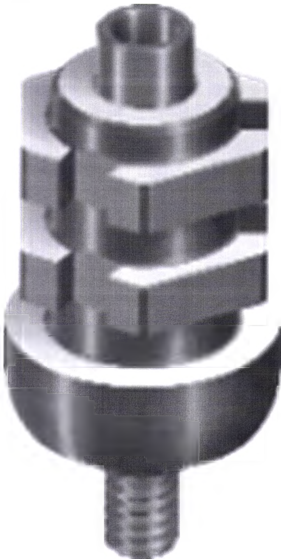
1.30. WN synOcta impression cap, screw-retained, with integral guide screw, H 10mm, артикульный номер 048.091
