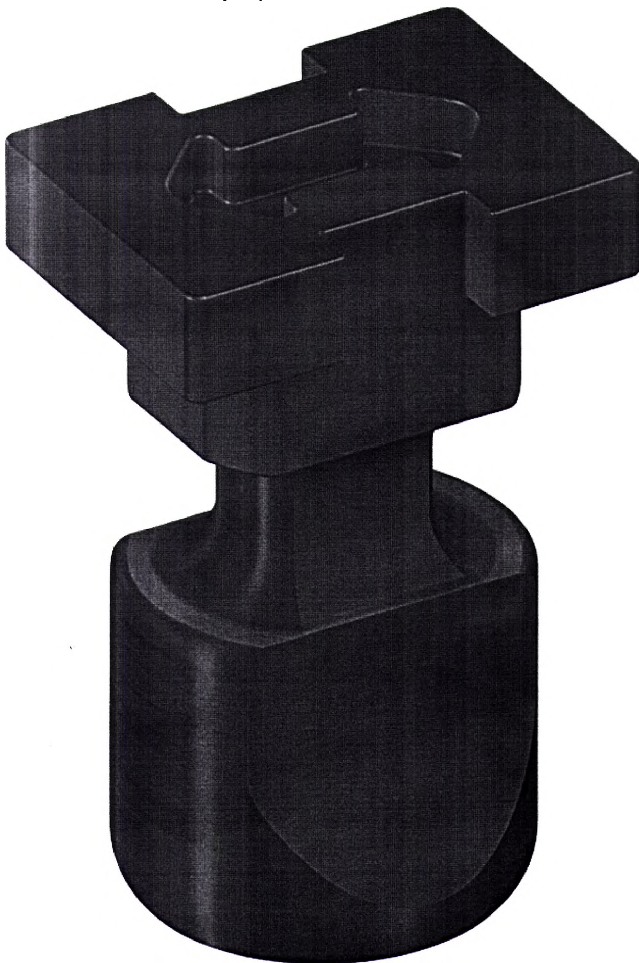
1.25. Impression post for closed tray, abutment level, for screw-retained abutment, D 4.6mm, артикульный номер 025.2246
