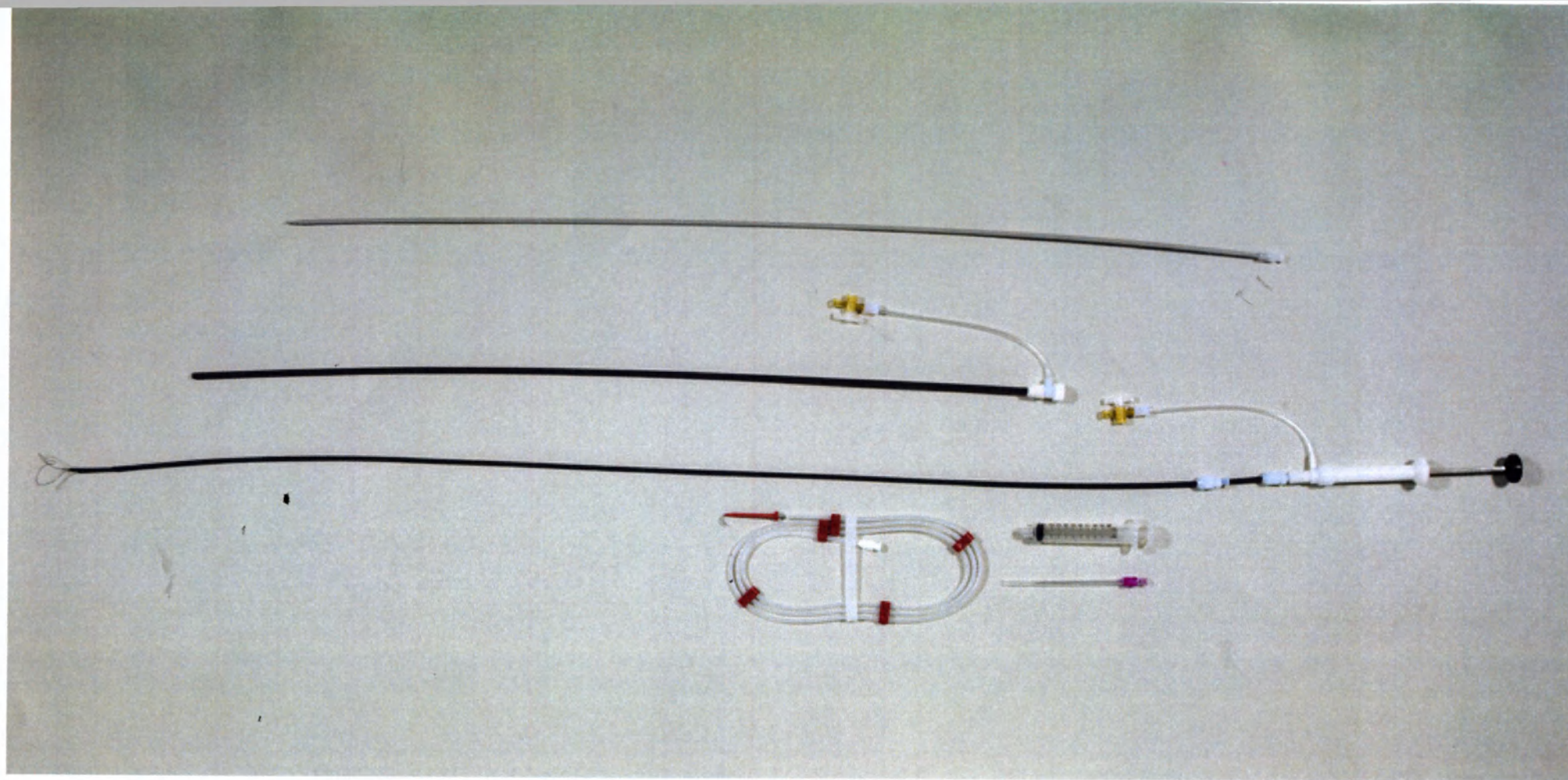
Ретриверы с петлей: LR-NES001, LR-NES002, LR-NES541, LR-SSN001, LR-SSN002
