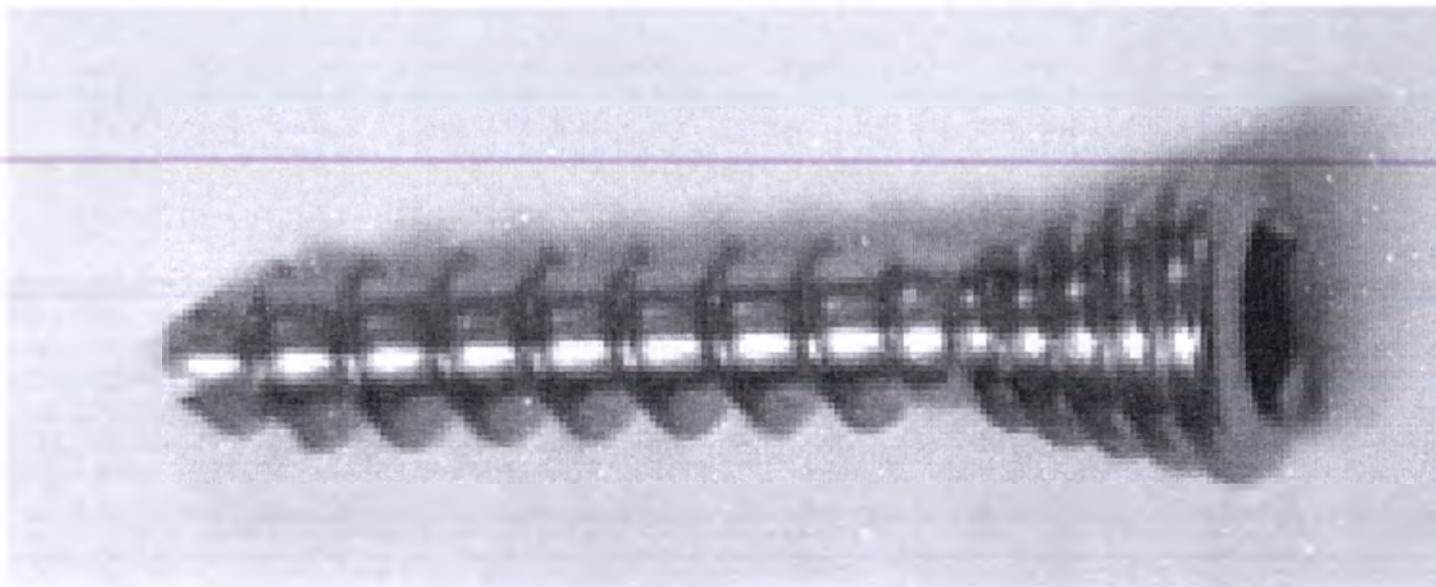
Винт ARIX Wrist System Bone Screw 161.052312.F;
