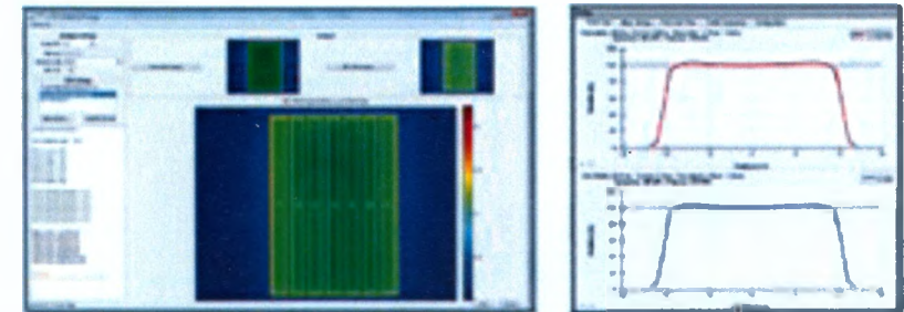
Check your MLC leaf errors, dose output and profiles, beam uniformity, constancy, flatness, and more
