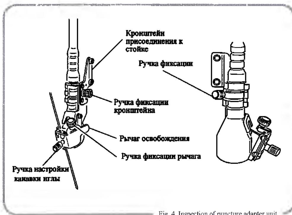
Fig. 4. Inspection of puncture adapter unit
