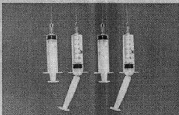
Self- destroyed Syringe
