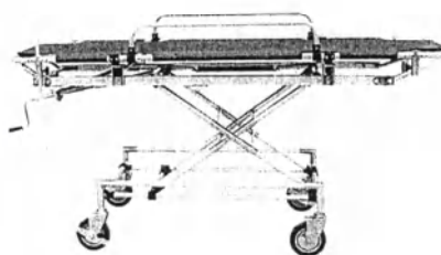
型号:BLQ030 多功能铝合金抢救推车 规格:1950 × 550 × 900 Type:BLQ030 multi-purpose aluminium alloy emergency trammer Specification:1950 × 550 × 900
