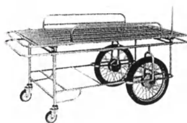
型号:BLQ029 全不锈钢两大轮、两小轮担架车 规格:1950 × 650 × 800 Type: BLQ029 full stainless steel litter carriage with two big wheels and two small wheels Specification:1950 × 650 × 800
